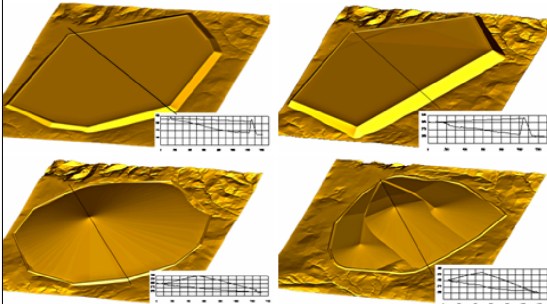
Figure 1: Typical TSF configurations
