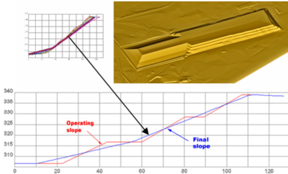
Figure 23: Development of a two-slope concave profile
