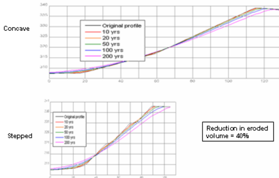
Figure 25: Comparison of erosion from a two-slope concave vs a stepped slope
