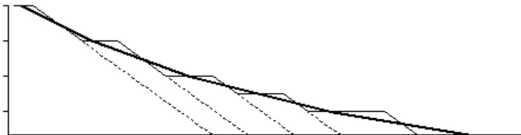
Figure 22: Stepped profile to achieve concave profile with minimum dozing
