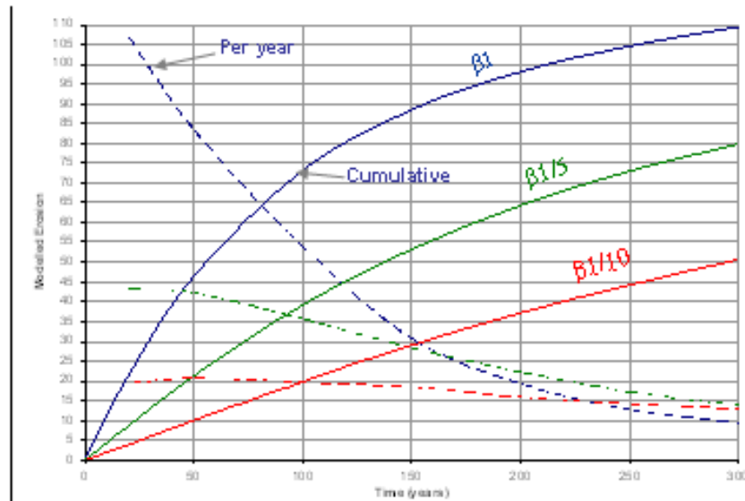
Figure 11: Influence of armouring - reduced erosion parameters
